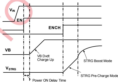
Figure 3: Charging Process when EN and ENCH Separated
